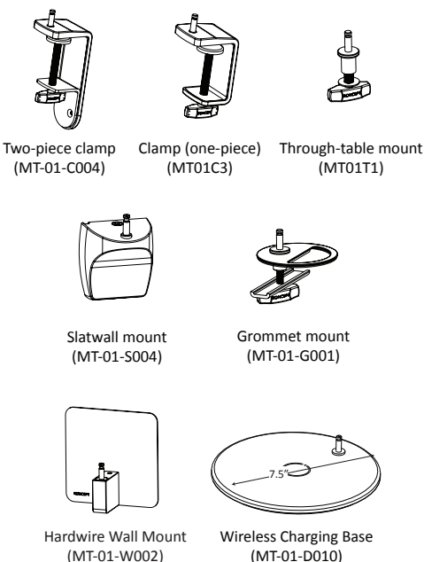
Mounting Options for Splitty Desk Lamp***
