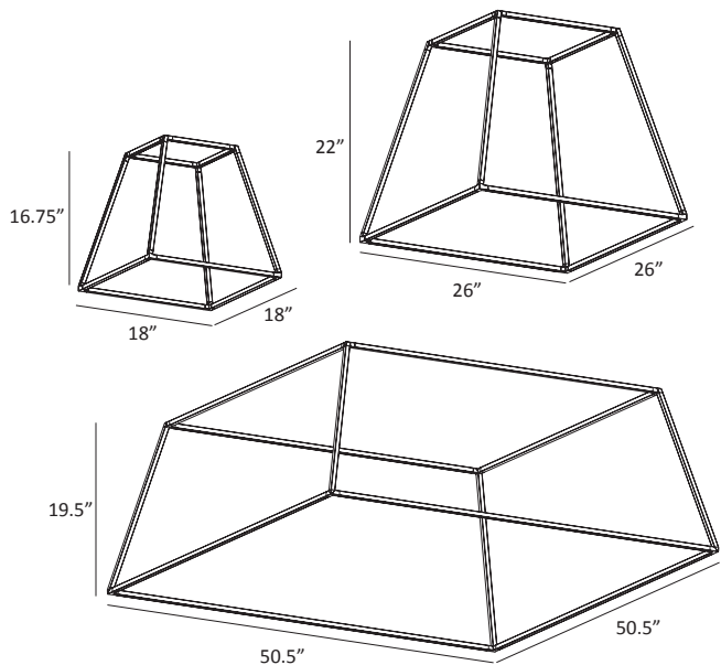
Z-Bar Rise Square
