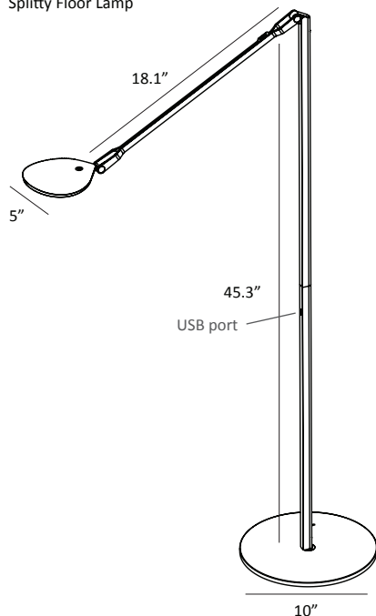
Splitty Floor Lamp
